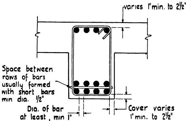
Fig. 244. —Sketch showing Minimum Covers required.
